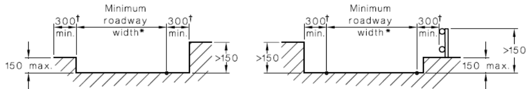
(c) High obstruction on one side of roadway (d) High obstruction on both sides of roadway
