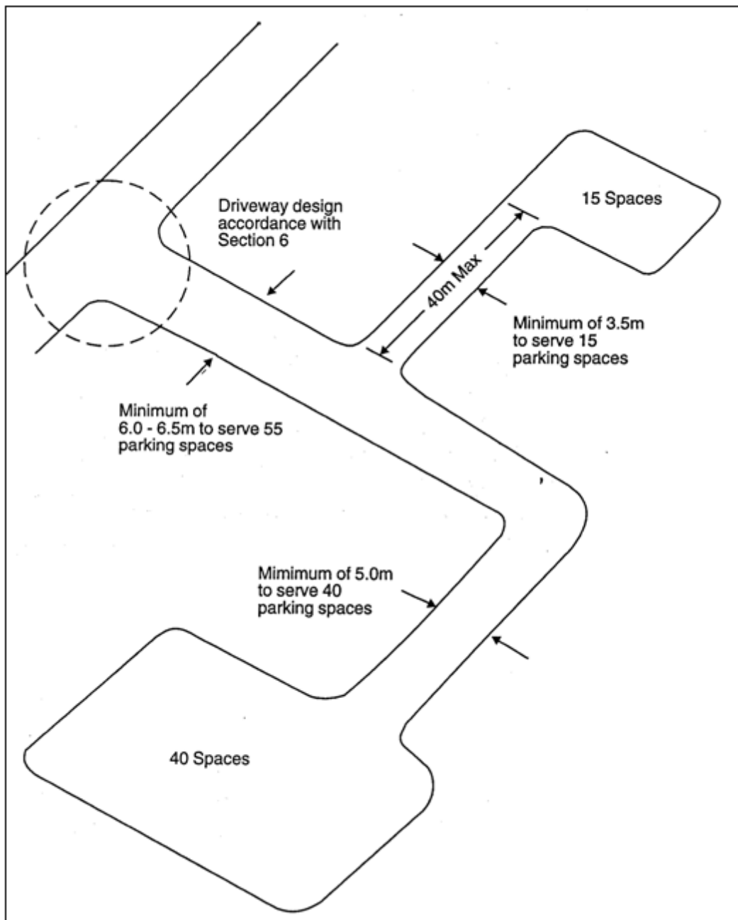
Figure 14 Car parking layout
