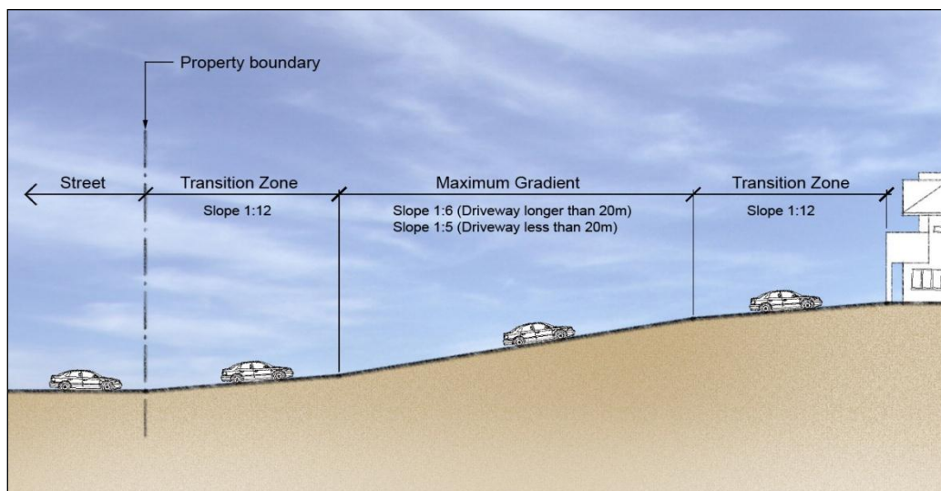
Figure 15 Driveway gradients
